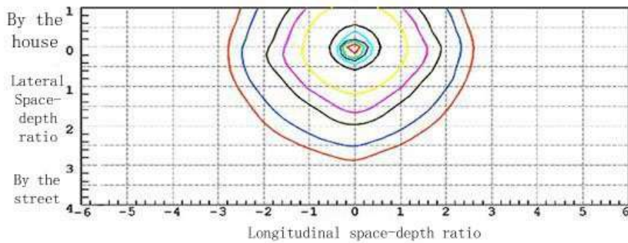
Absolute illumination curve of horizontal plane
