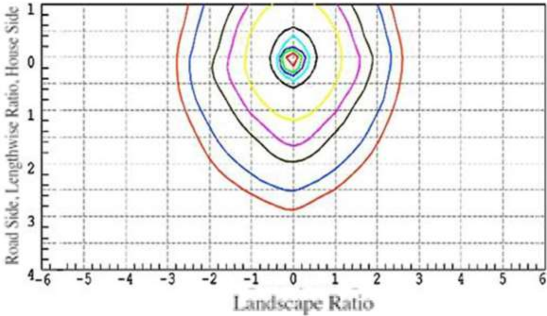
Horizontal Absolute Illumination Curve
